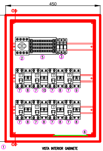
VISTA INTERIOR GABINETE
