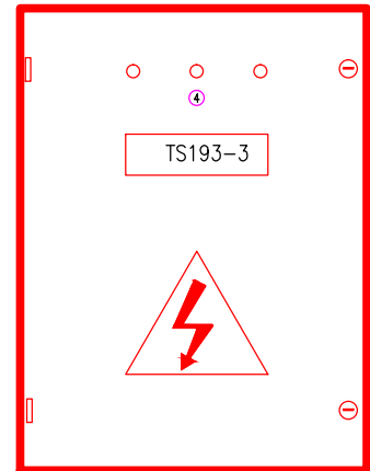
VISTA FRONTAL GABINETE
